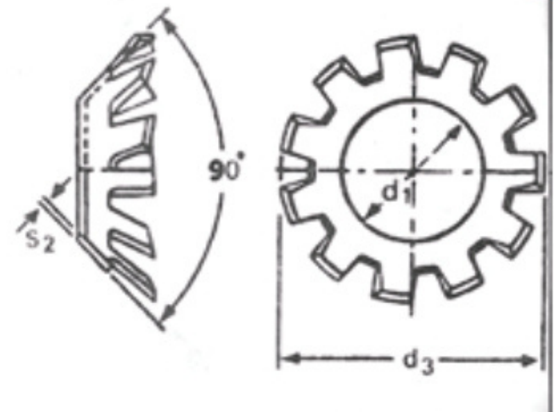
Type C: Countersunk
