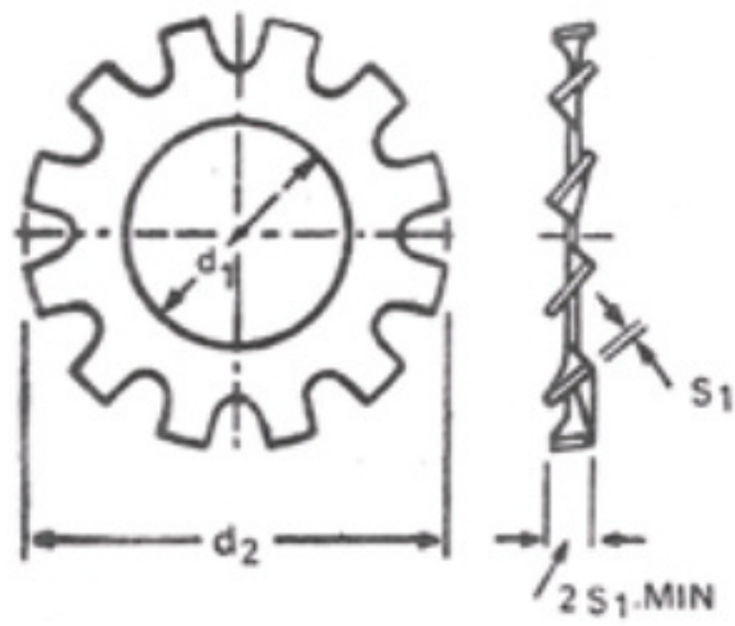
Type A: Externally Toothed T
