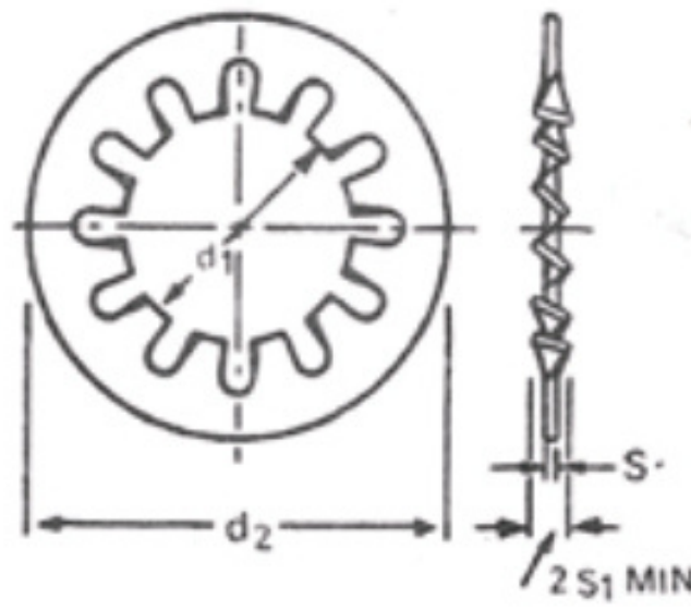
Type B: Internally Toothed
